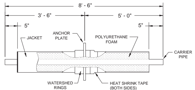
ANCHOR DETAIL
