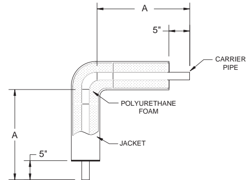
90° ELBOW DETAIL
