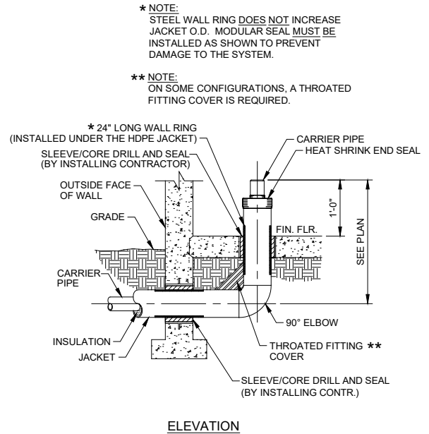
BUILDING RISER DETAIL SCALE: NONE
