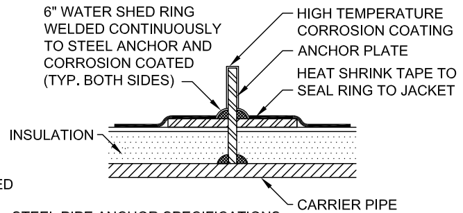
STEEL PIPE ANCHOR SPECIFICATIONS
